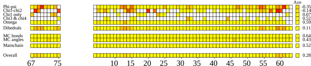
g. G-factors
