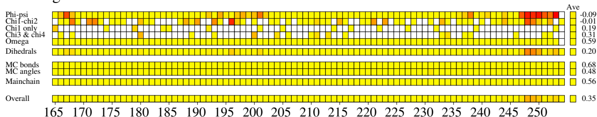
g. G-factors
