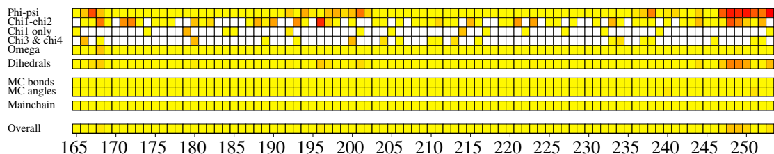
g. G-factors
